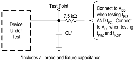
Figure 7. Test Circuit
