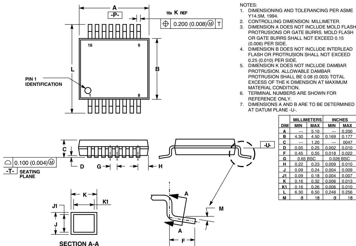
Figure 37. Outline Dimensions for DT Suffix, TSSOP-16 (Case 948C-03, Issue B)
